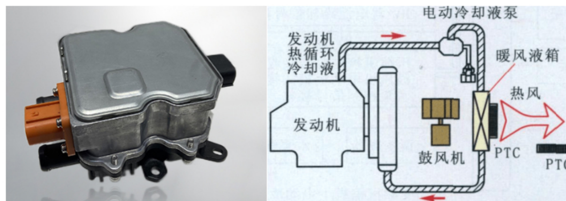
Automotive PTC
