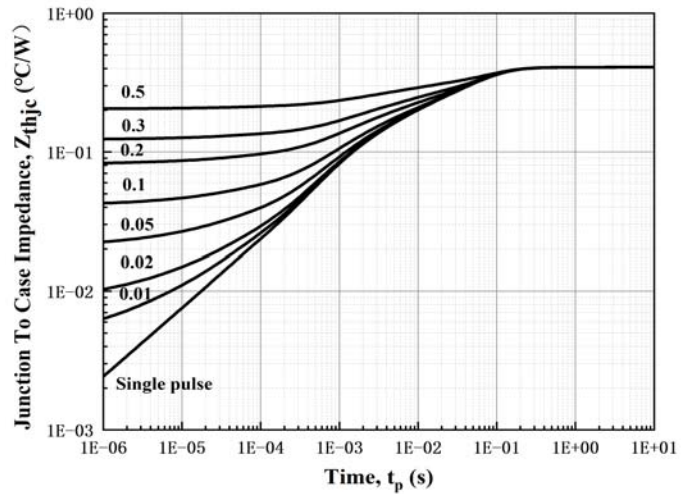
Figure 18 Transient Thermal Impedance (Junction - Case)
